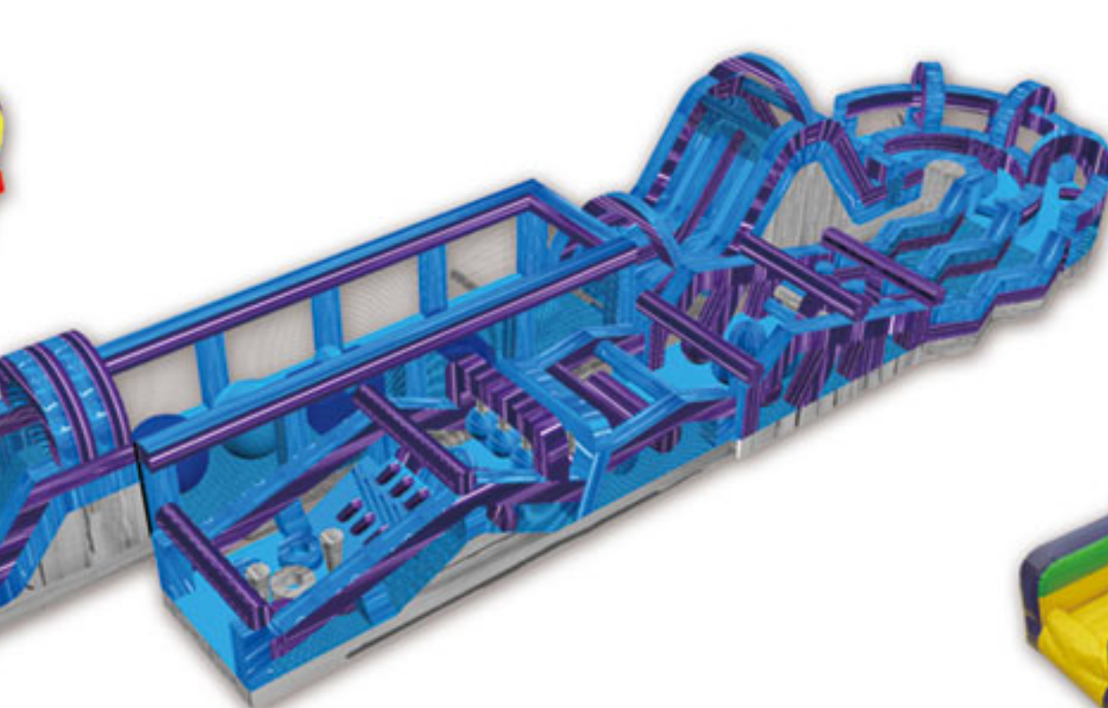
⓭ Mega Obstacle Run-Marble Purple (1+2+3+5+4) Blowers ..... 4-1.5HP & 1-2.0+HP Inflated DIMS ..... 95' L x 26' W x 16' H Platform height ..... 9' Game Weight ..... 1,994 lbs.
